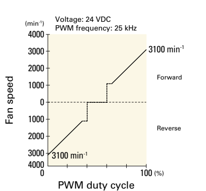
PWM duty - Speed characteristics example
